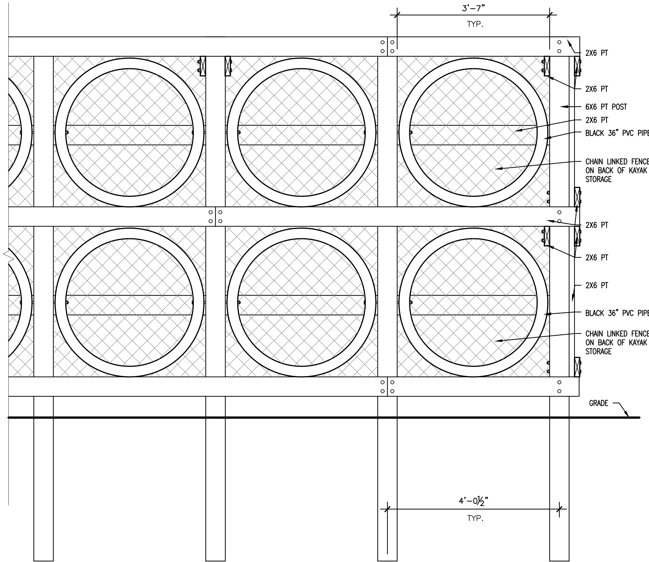
5 PROPOSED SECTION 3/4" = 1'-0"
