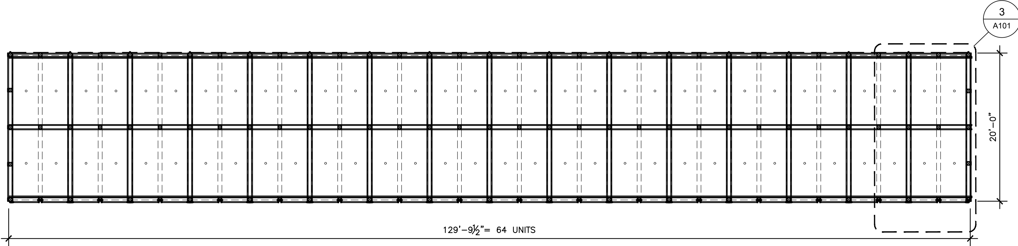
1 LARGE KAYAK STORAGE PLAN A101 1/8" = 1'-0"
