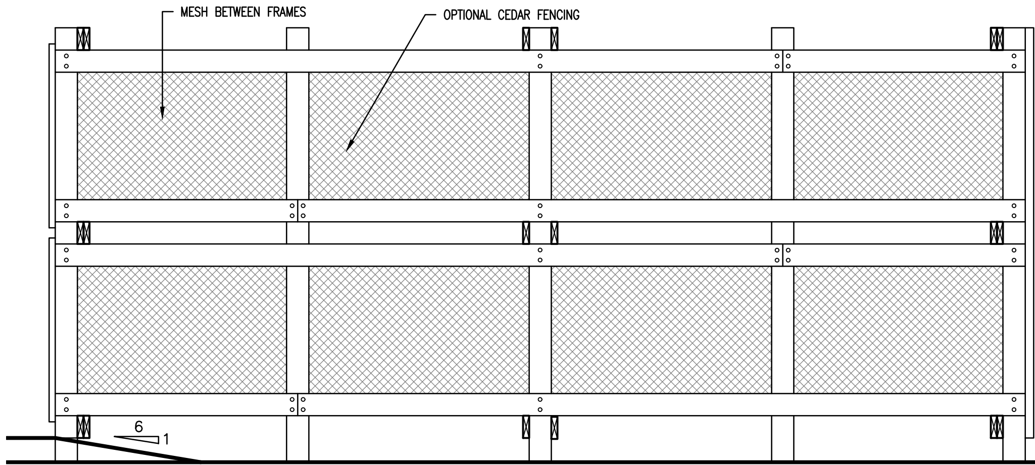
8 SIDE ELEVATION A101 1/2" = 1'-0"
