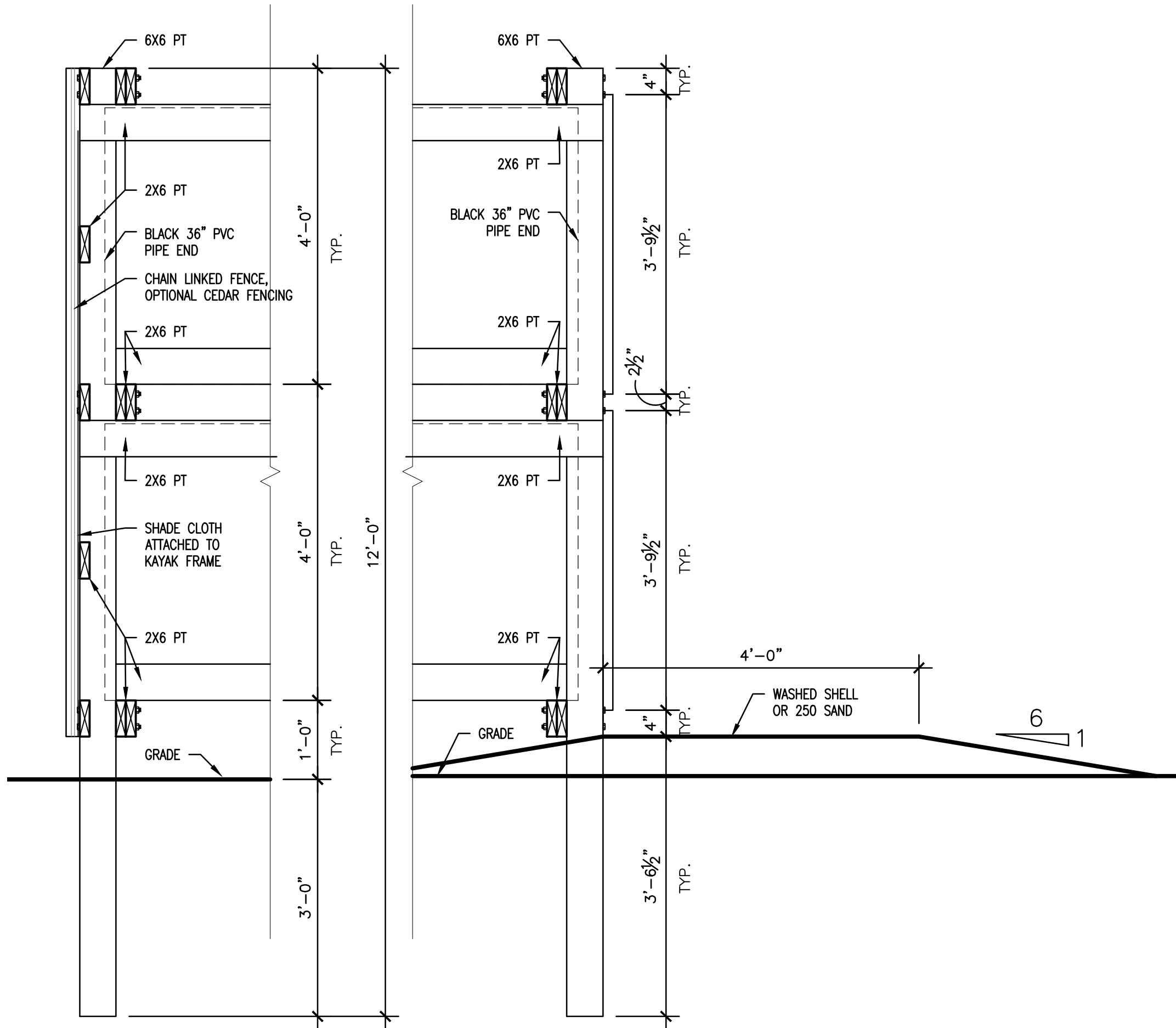
4 PROPOSED SECTION 3/4" = 1'-0"
