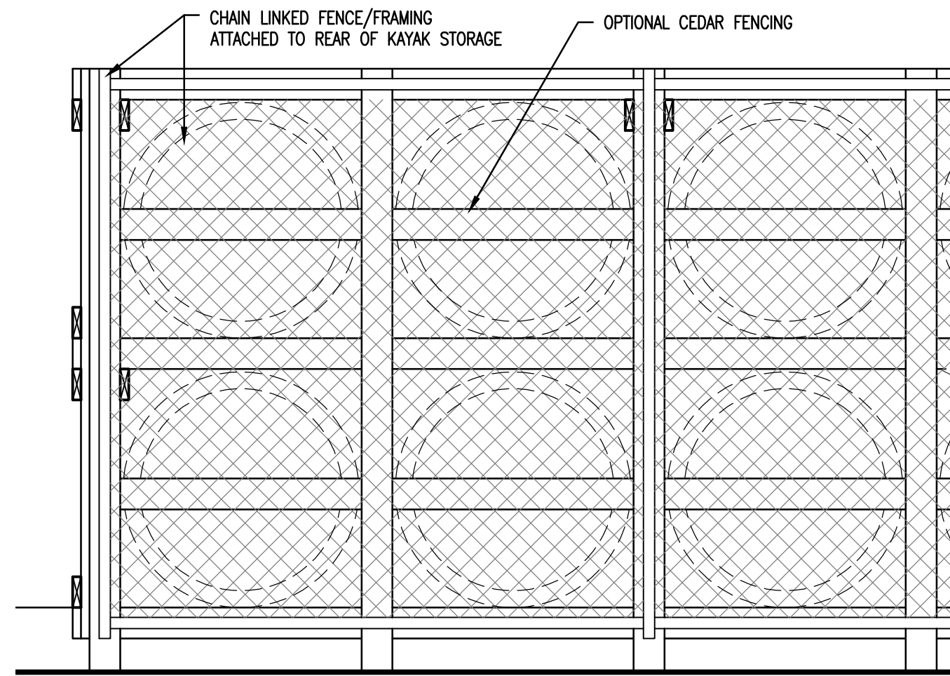
9 REAR ELEVATION A101 1/2" = 1'-0"
