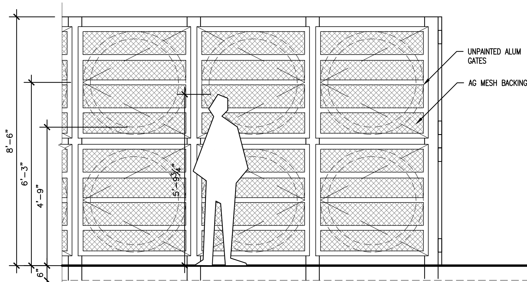
7 FRONT ELEVATION A101 1/2" = 1'-0"
