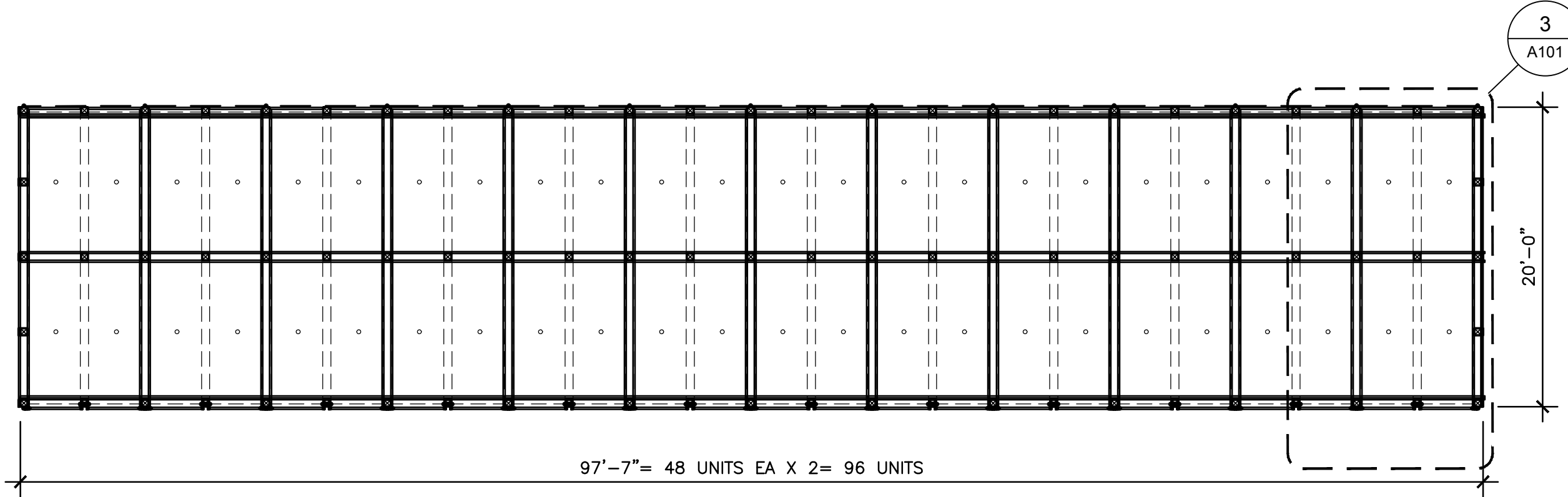
2 SMALL KAYAK STORAGE PLAN A101 1/8" = 1'-0"
