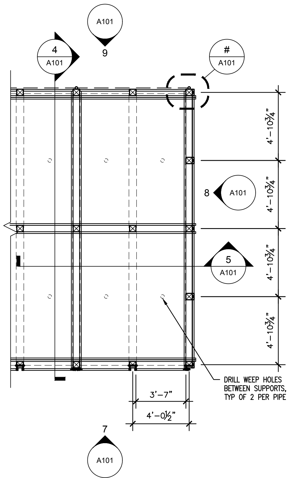
3 PROPOSED ENLARGED PLAN A101 1/4" = 1'-0"
