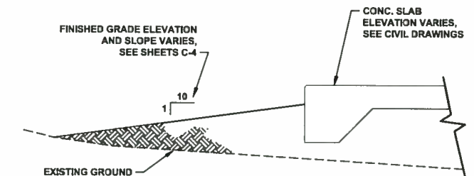
6 GRADING AT CONCRETE SLAB DETAIL C-3
