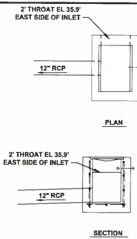
2 DRAINAGE STRUCTURE DETAILS AND ELEVATIONS C-12 NTS
