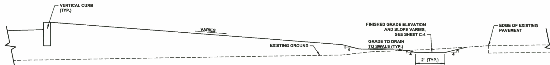
B SWALE DETAIL SECTION B-B C-4
