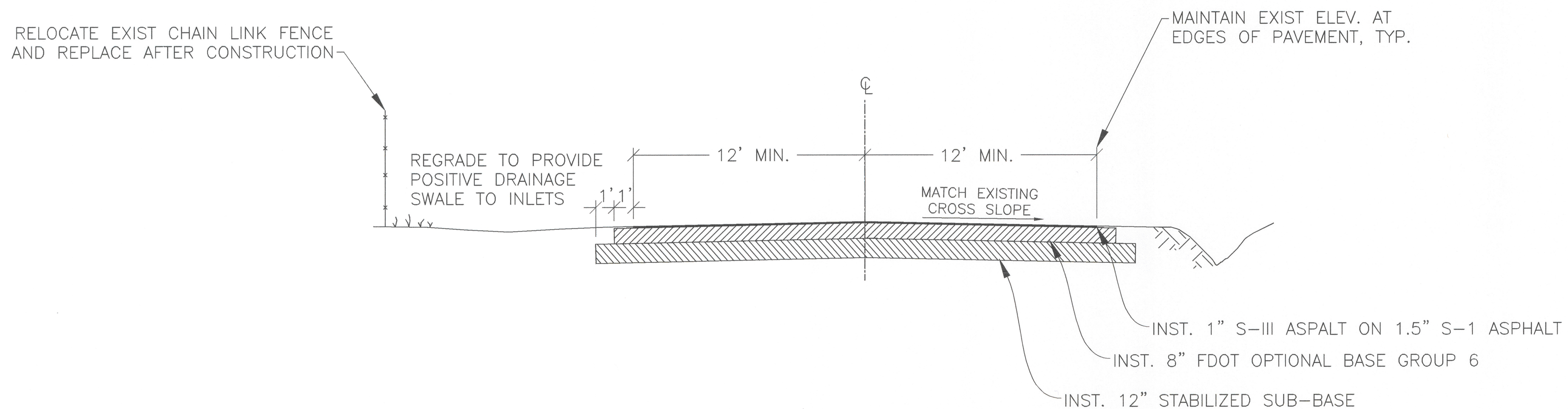
PROPOSED TYPICAL SECTION-65TH STREET WEST- LOOKING NORTH
