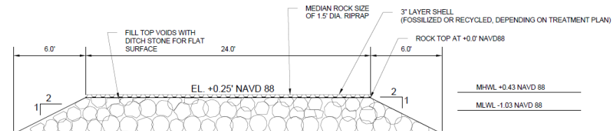
A TYPICAL RIPRAP MODULE PROFILE VIEW CM-3.1 (TREATMENTS A AND B) SCALE 1" = 4'
