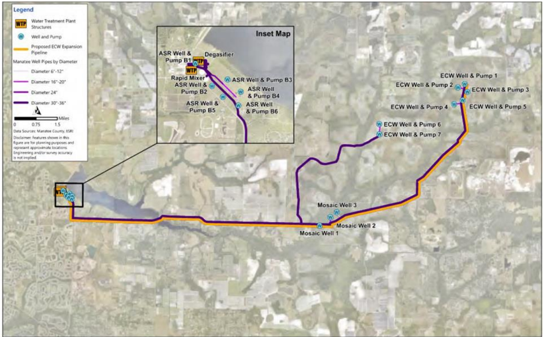
Figure 2 East County Wellfield and Pipeline Alignment Map with Proposed ECW Expansion Pipeline
