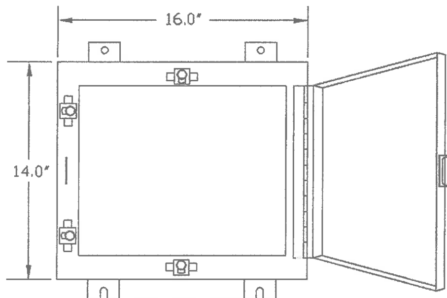
JUNCTION BOX (POWDER COATED WHITE)
