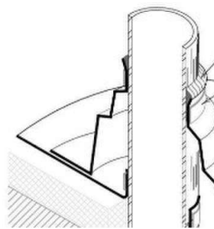
Stack Vent Flashing Isometric Detail
