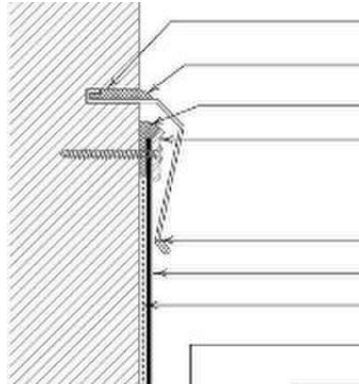
Flashing at Parapet Wall Detail
