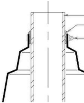
Stack Vent Flashing Detail
