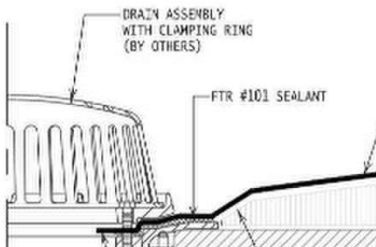
Drain Flashing Detail
