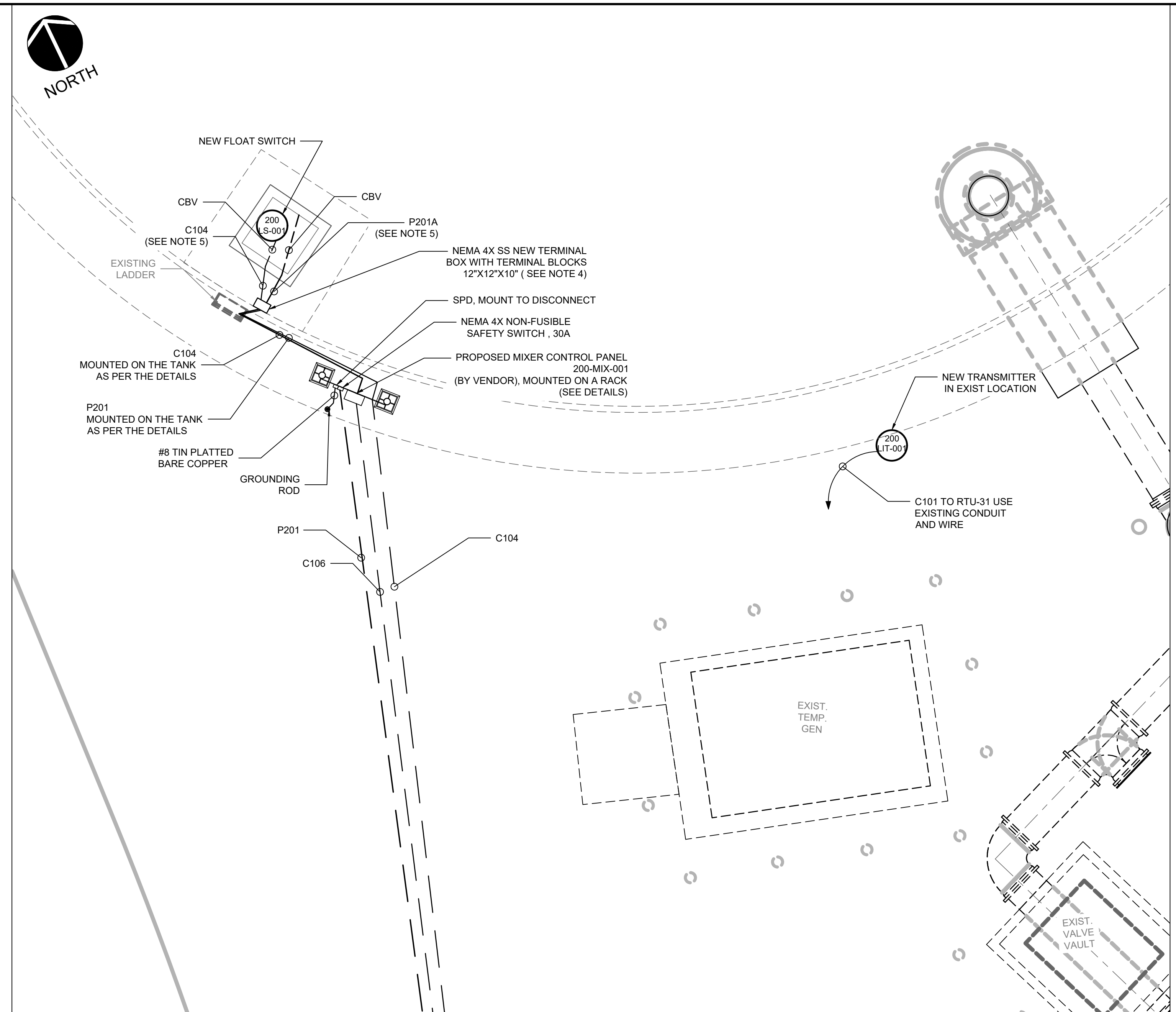
PROPOSED PARTIAL ELECTRICAL SITE PLAN 1
