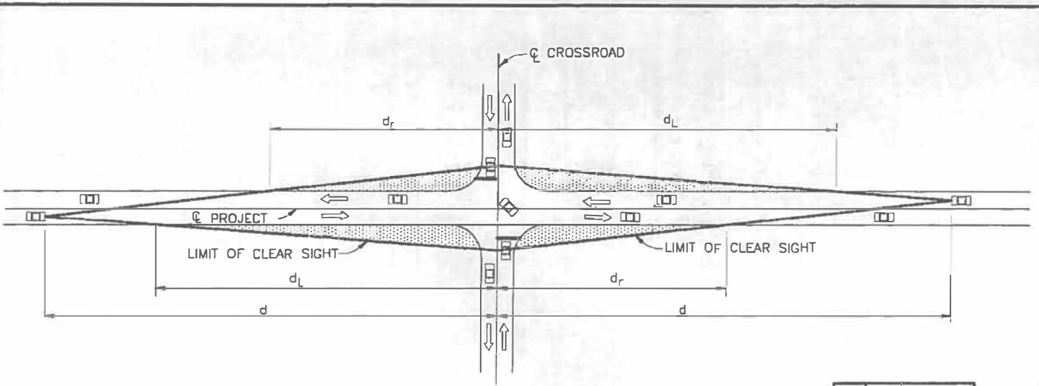
SIGHT WINDOW DETAIL
