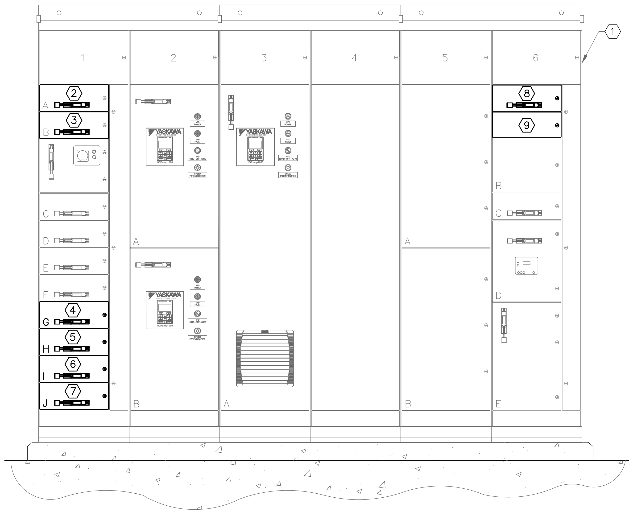
PROPOSED SEPTAGE AND GREASE RECIEVING MCC FRONT ELEVATION
