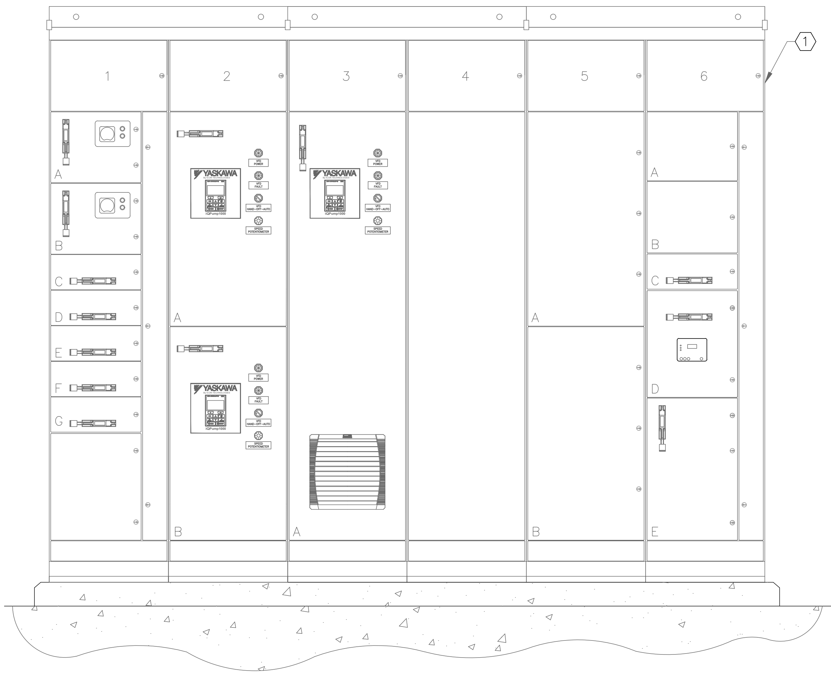
EXISTING SEPTAGE AND GREASE RECIEVING MCC FRONT ELEVATION
